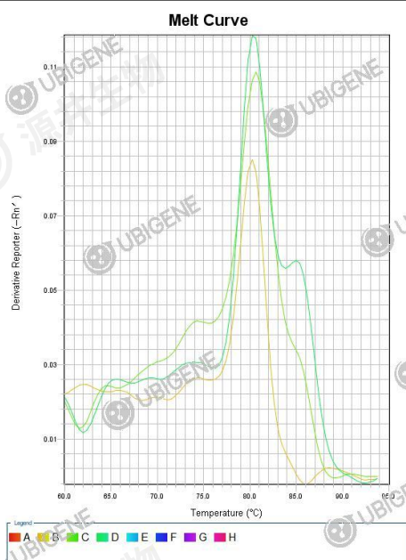
HFF-1_Ctrl(Puro)+hELN-1 melt curve
