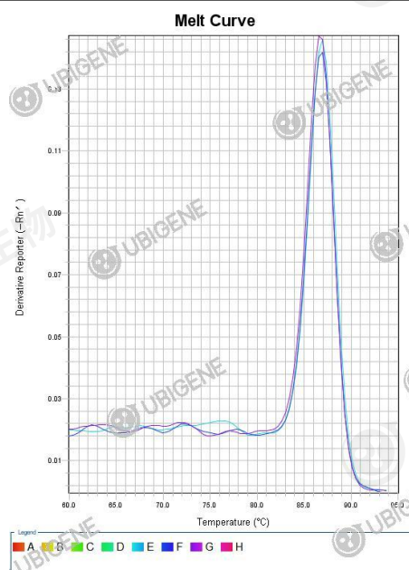
HFF-1_Ctrl(Puro)+ \beta -h_actin melt curve
