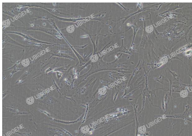
ELN Stable Expression Cell Line (HFF-1)-100X
