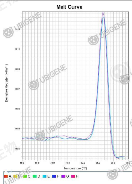
ELN Stable Expression Cell Line (HFF-1)+ \beta -h_actin melt curve
